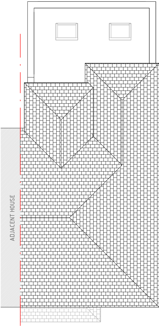
05/304 – PROPOSED ROOF PLAN 1 : 100
