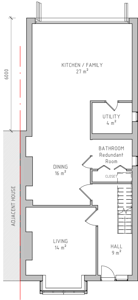
05/301 – PROPOSED GROUND FLOOR PLAN 1 : 100
