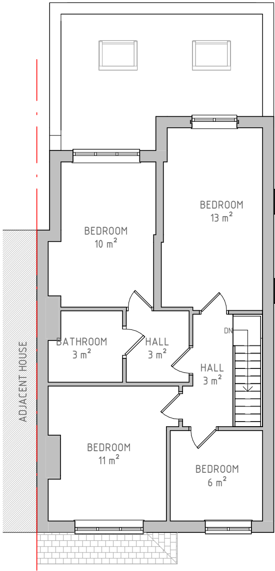
05/302 – PROPOSED FIRST FLOOR PLAN 1 : 100
