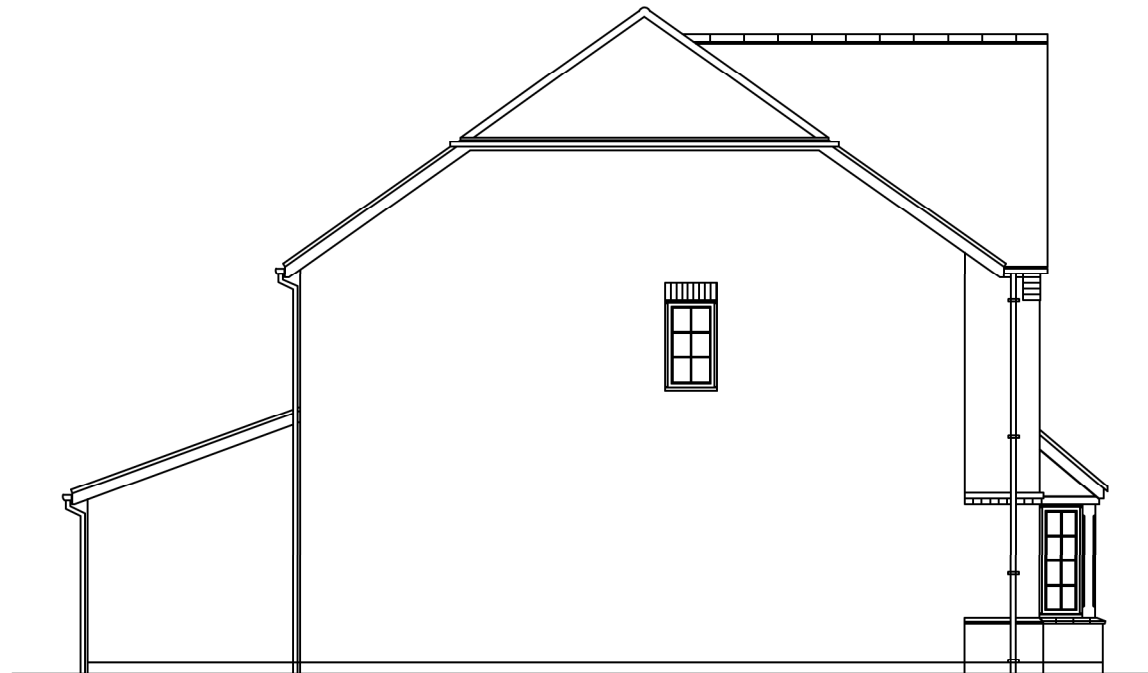
SIDE ELEVATION - Plots 9,10,16,48
