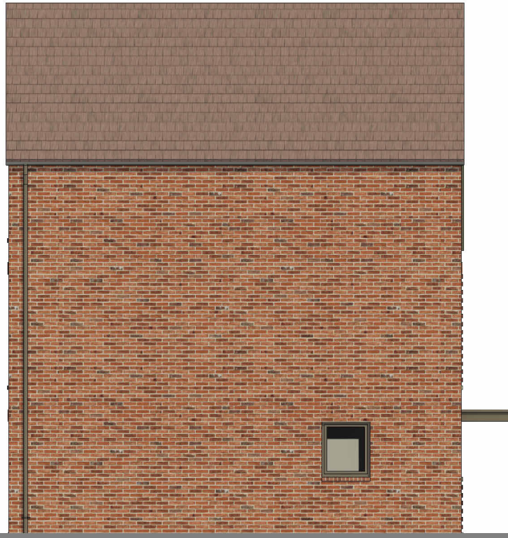
Left Elevation 1 : 100
