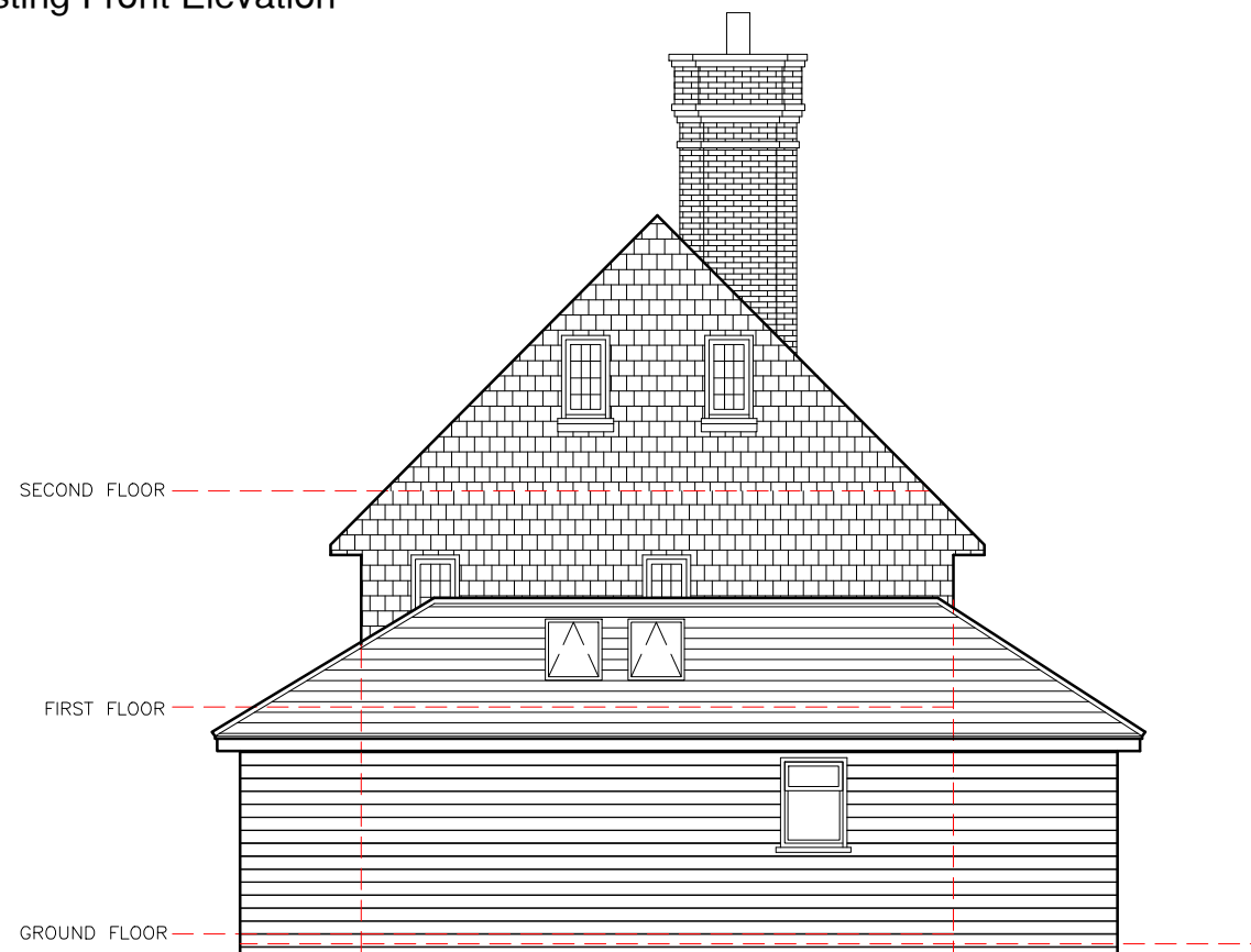
A) Existing Front Elevation
