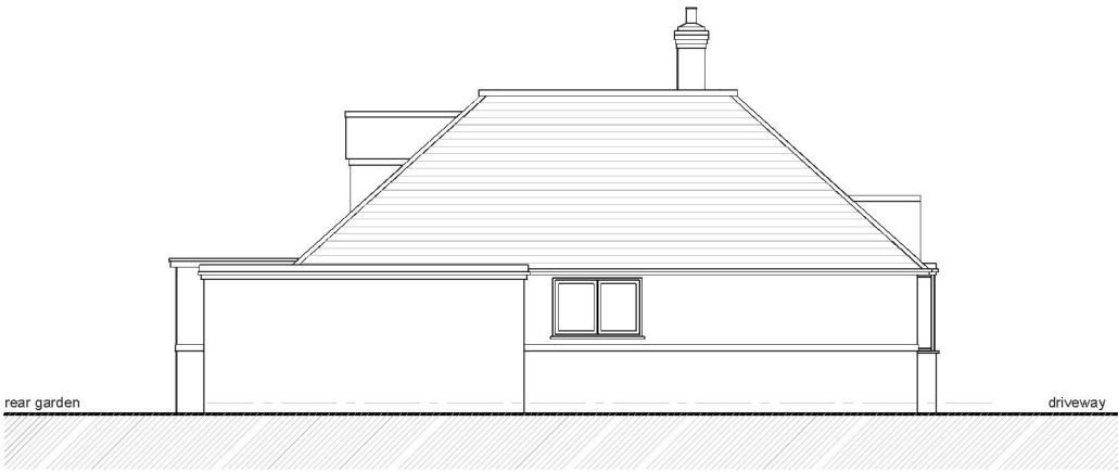
Flank Elevation (South)
