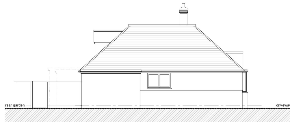
Flank Elevation (South)
