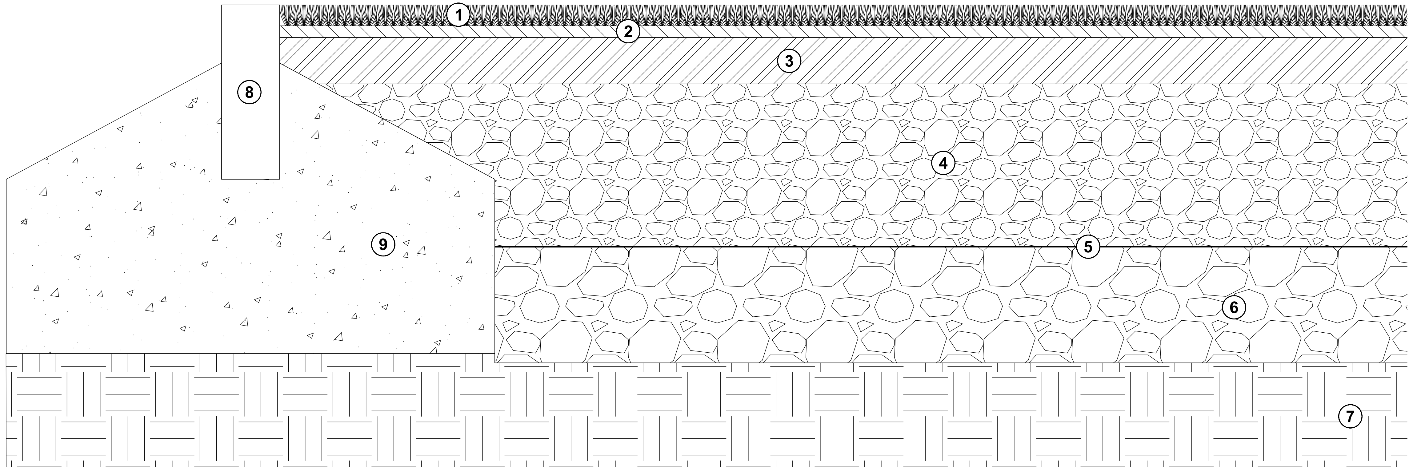
ARTIFICIAL HOCKEY TURF PITCH (HTP) CONSTRUCTION
