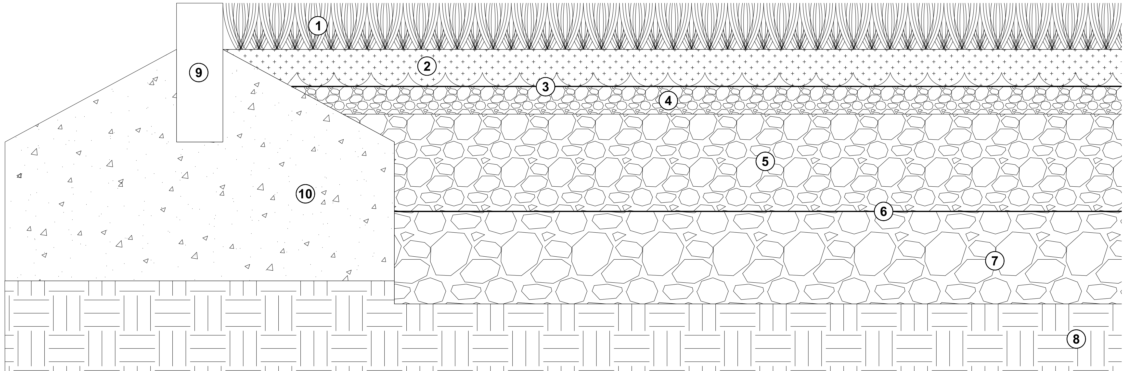
ARTIFICIAL GRASS PITCH (AGP) CONSTRUCTION
