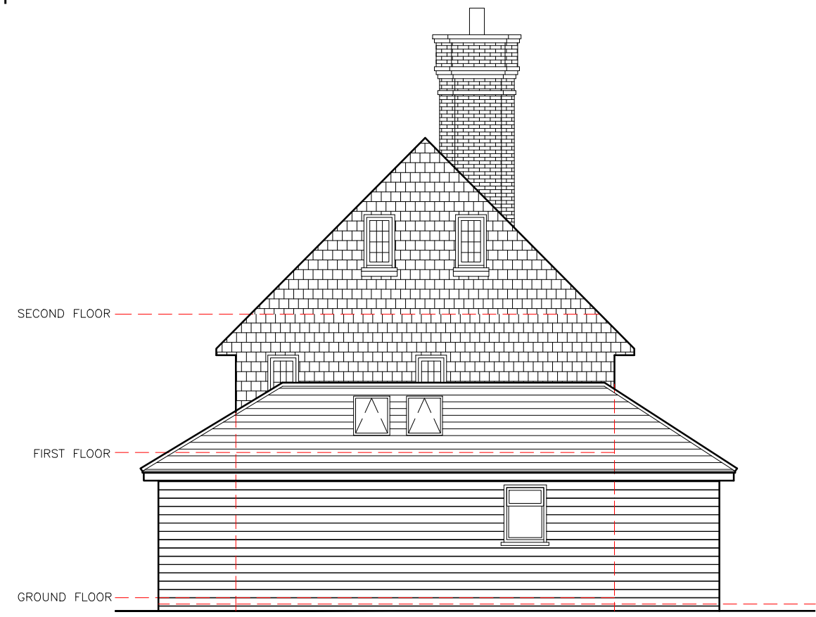
A) Proposed Front Elevation
