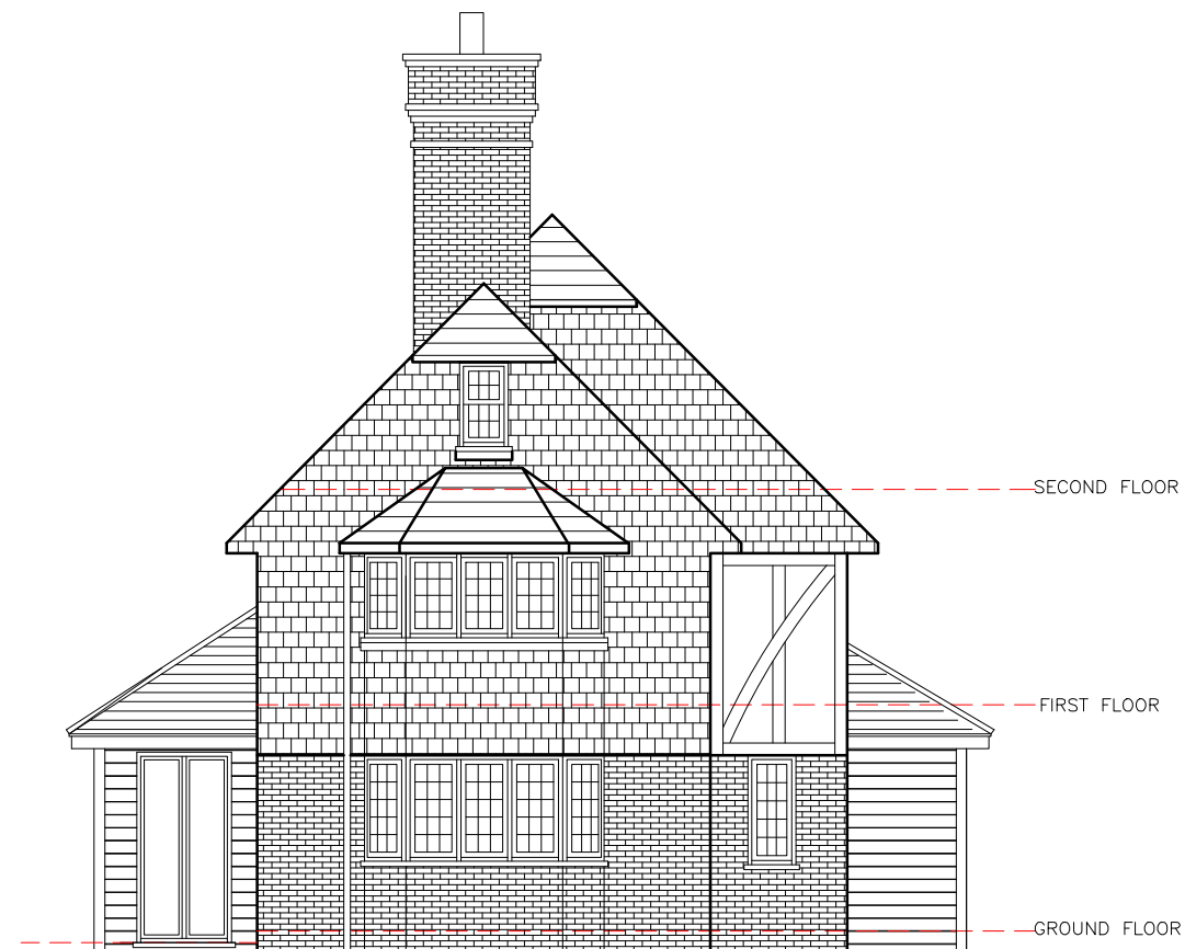
C) Proposed Rear Elevation
