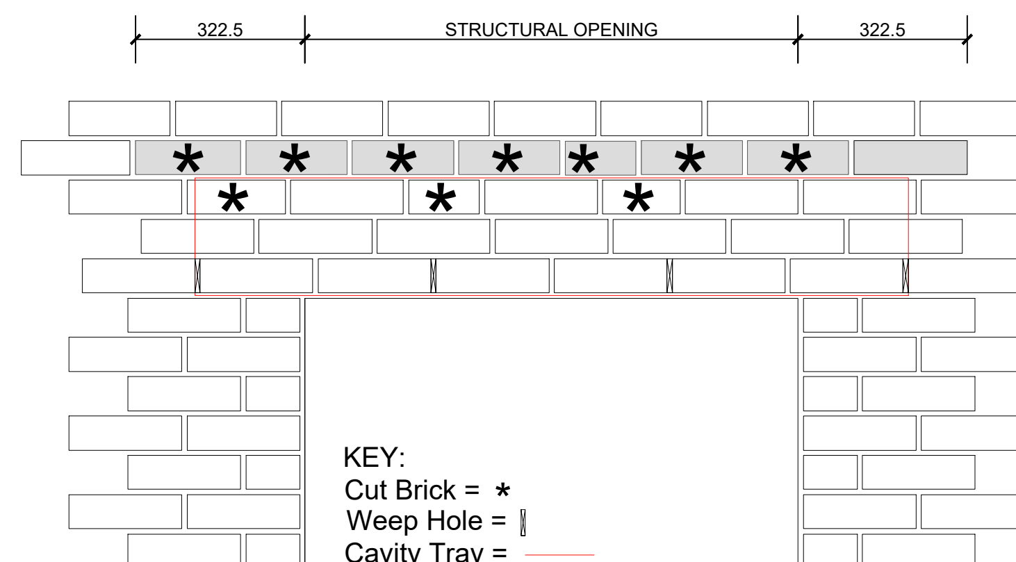
FEATURE HEAD TYPICAL SETTING OUT 1:10
