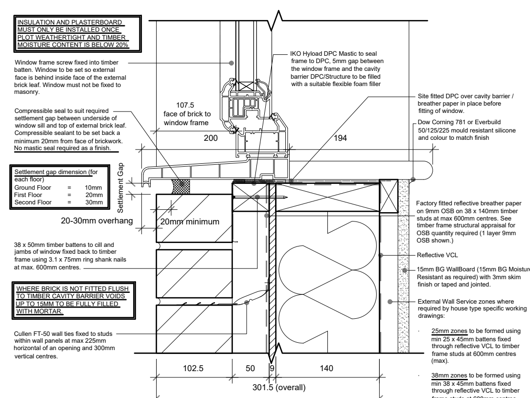
STANDARD CILL DETAIL 1:5
