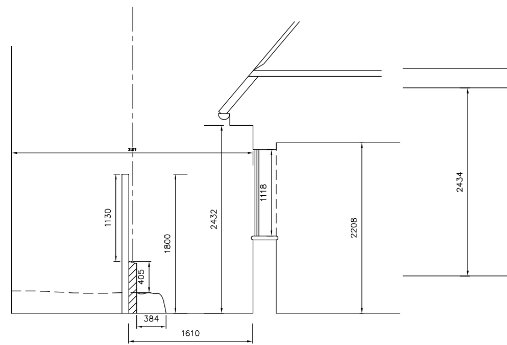
Side Section scale 1:50
