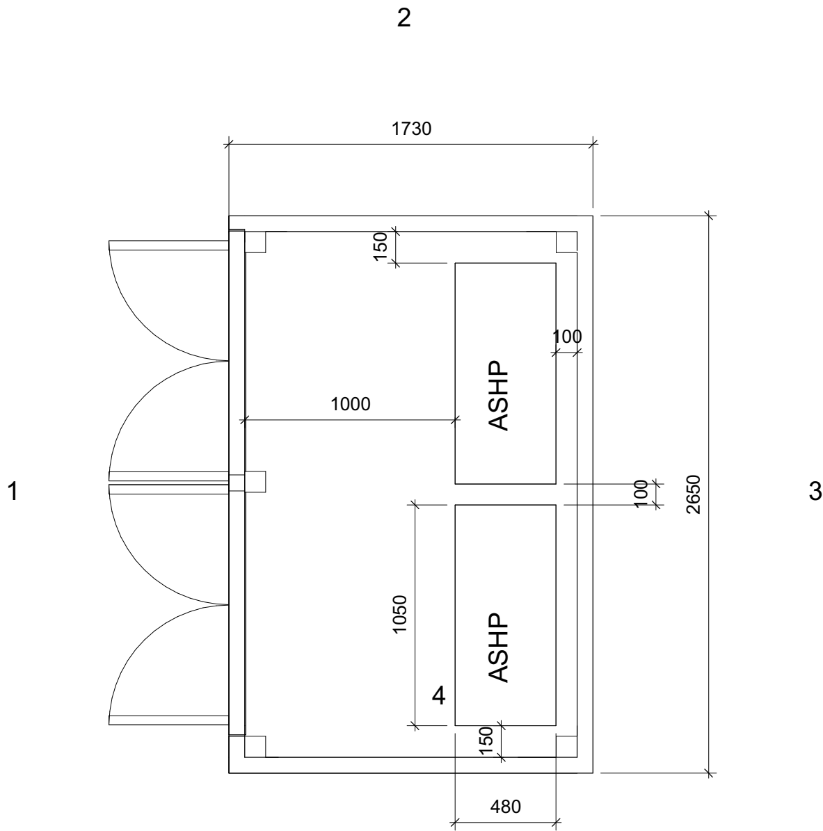
Enclosure type 2 Plan 1 : 25
