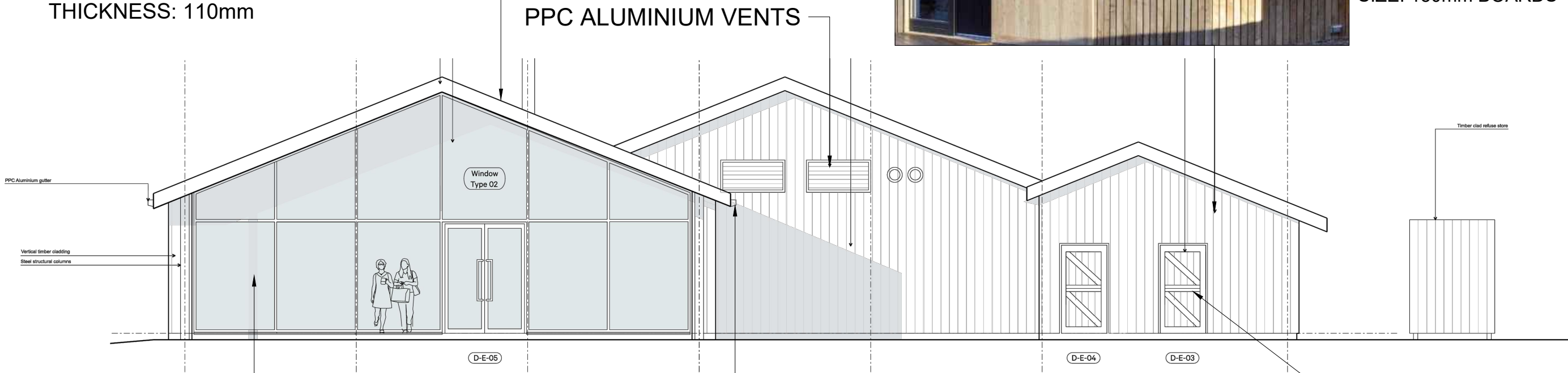
TIMBER CLADDING; PRODUCT; LARCH BOARD ON BOARD CLADDING COLOUR; 'UNCOATED', SIZE: 150mm BOARDS
