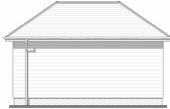
Side Elevation
