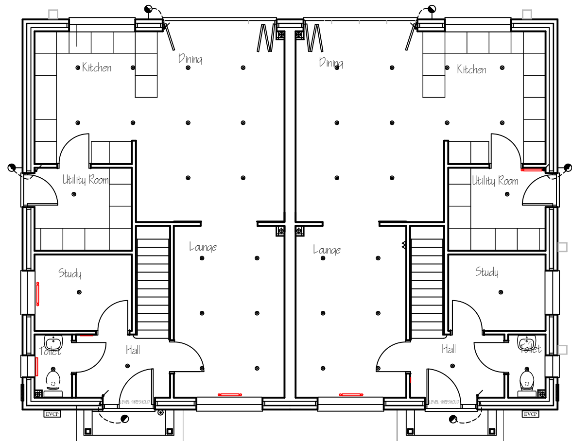
PROPOSED GROUND FLOOR LIGHTING LAYOUT
