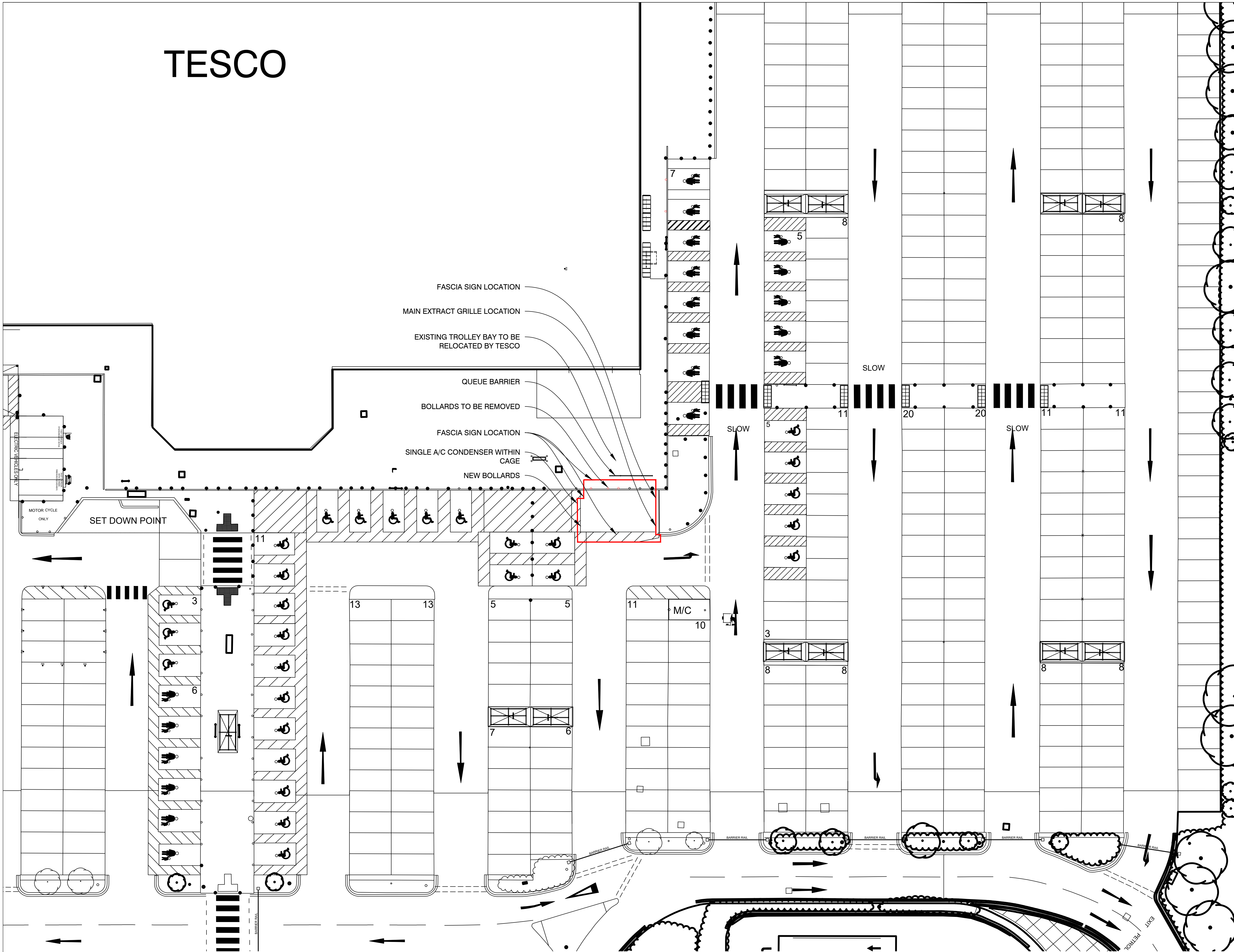
BLOCK PLAN (1:200)
