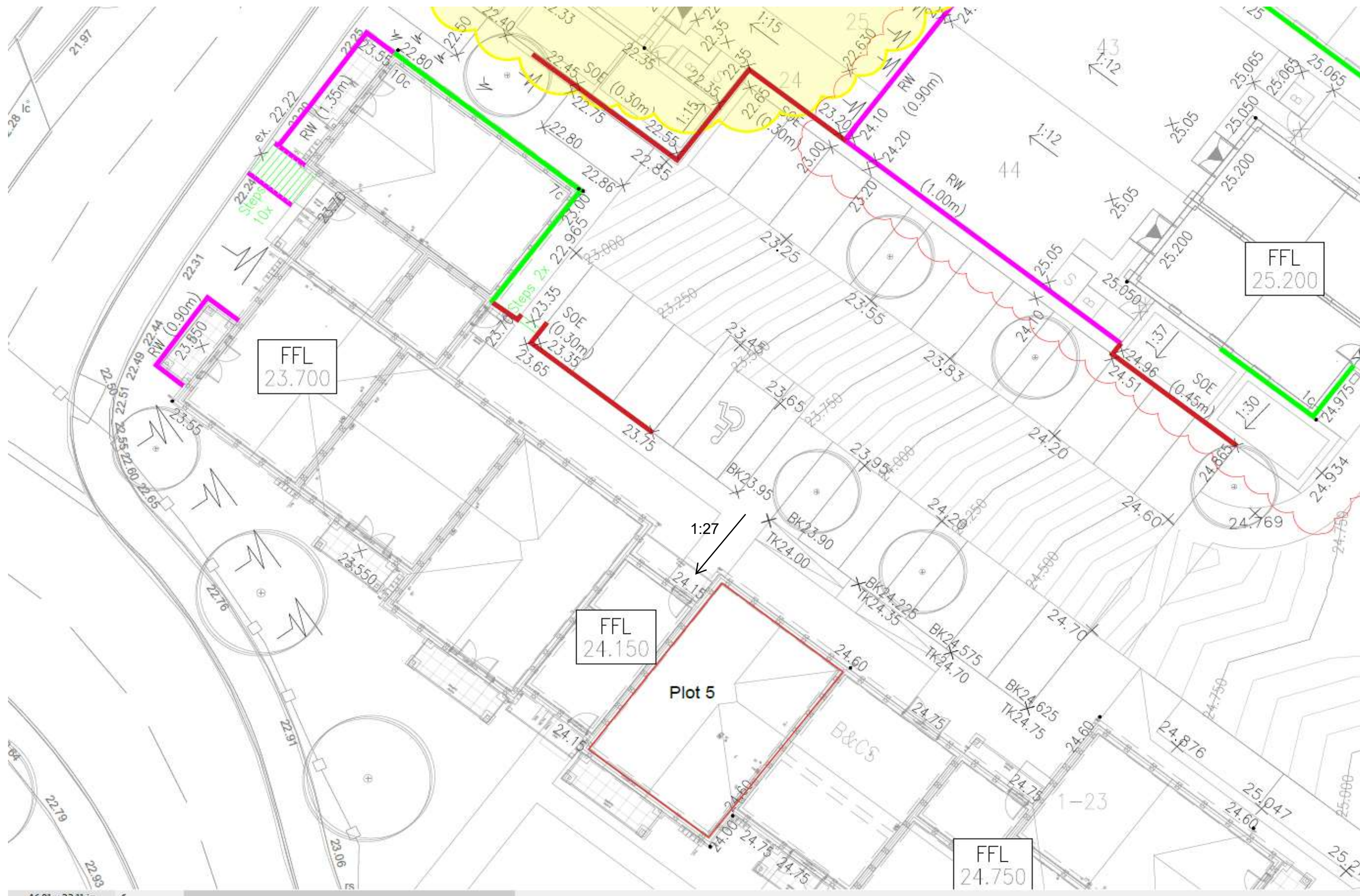
Part external works plan showing access around Plot 5 including gradients.
