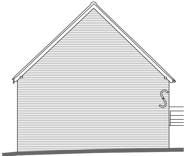
rear elevation north
