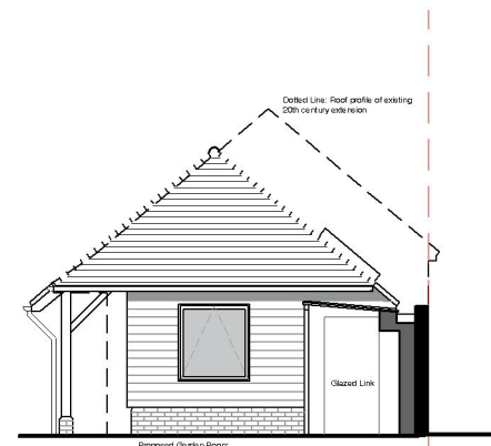
Section through Glazed Link (East View)
