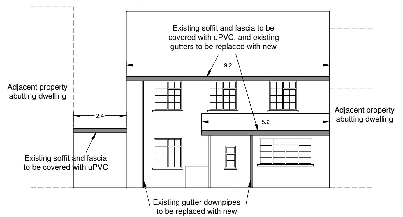
Rear Elevation
