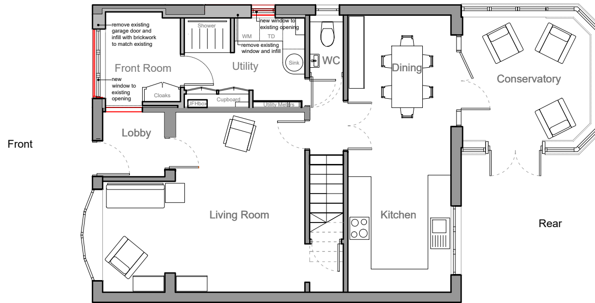
Proposed Plan - Ground Floor
