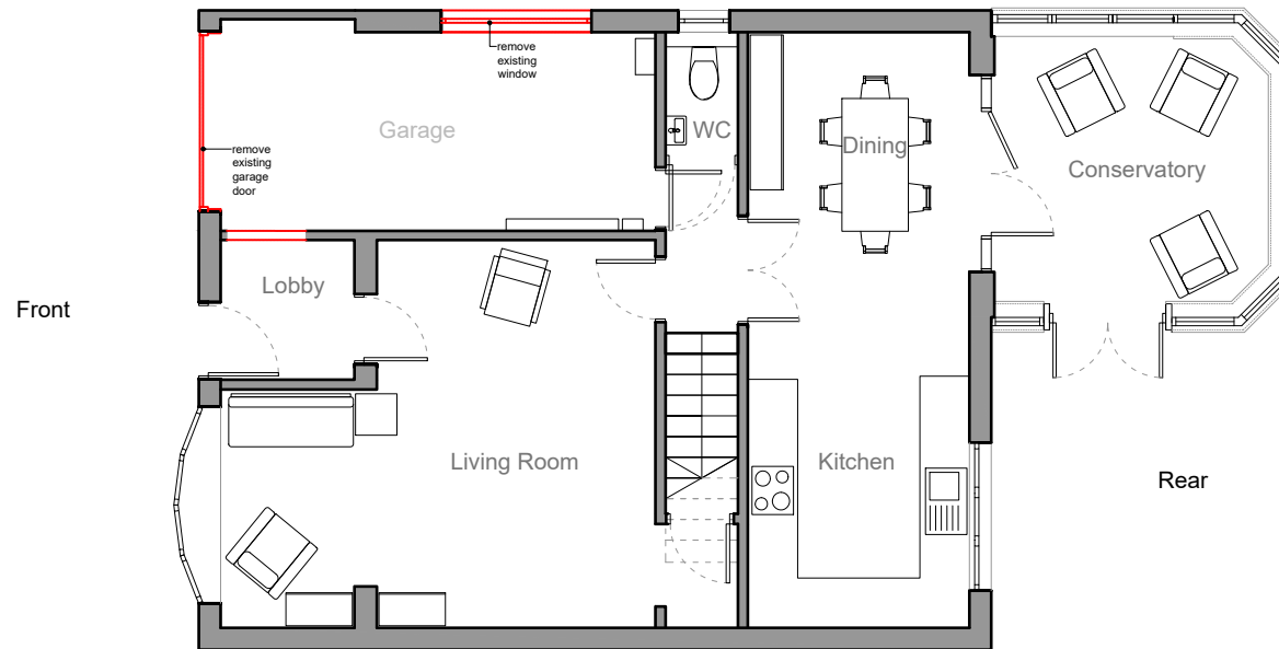
Existing Plan- Ground Floor
