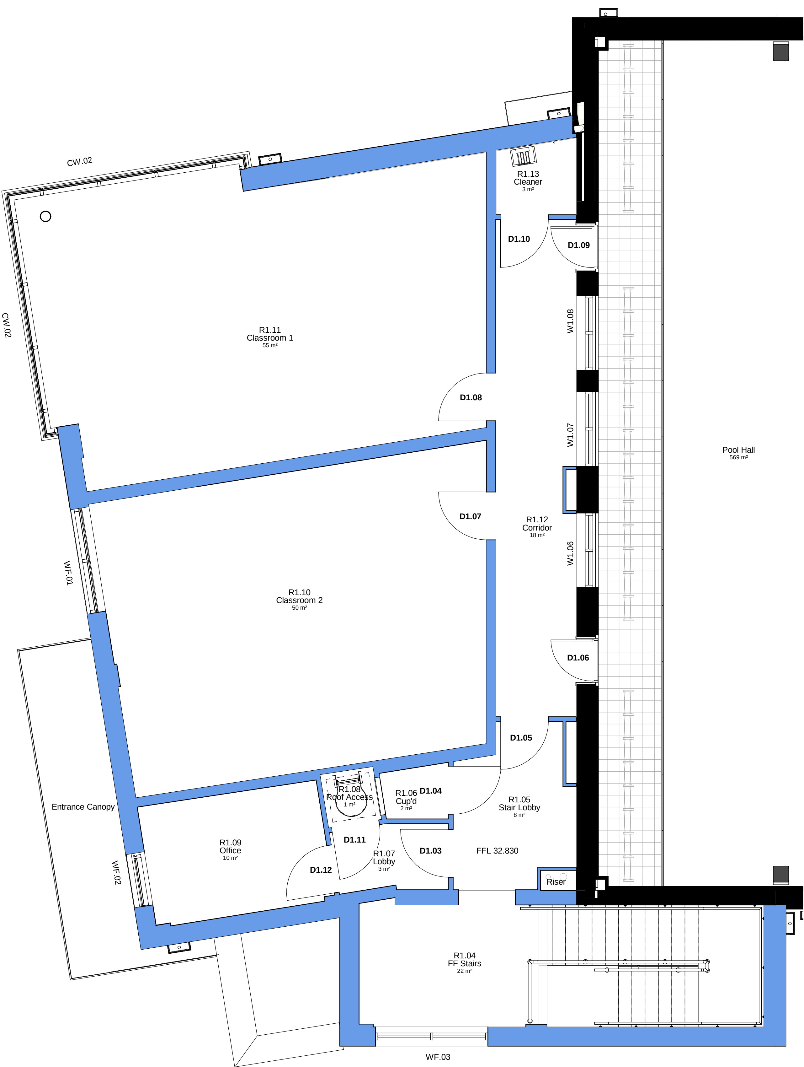
First Floor Detailed Classroom End Planning 1 : 50
