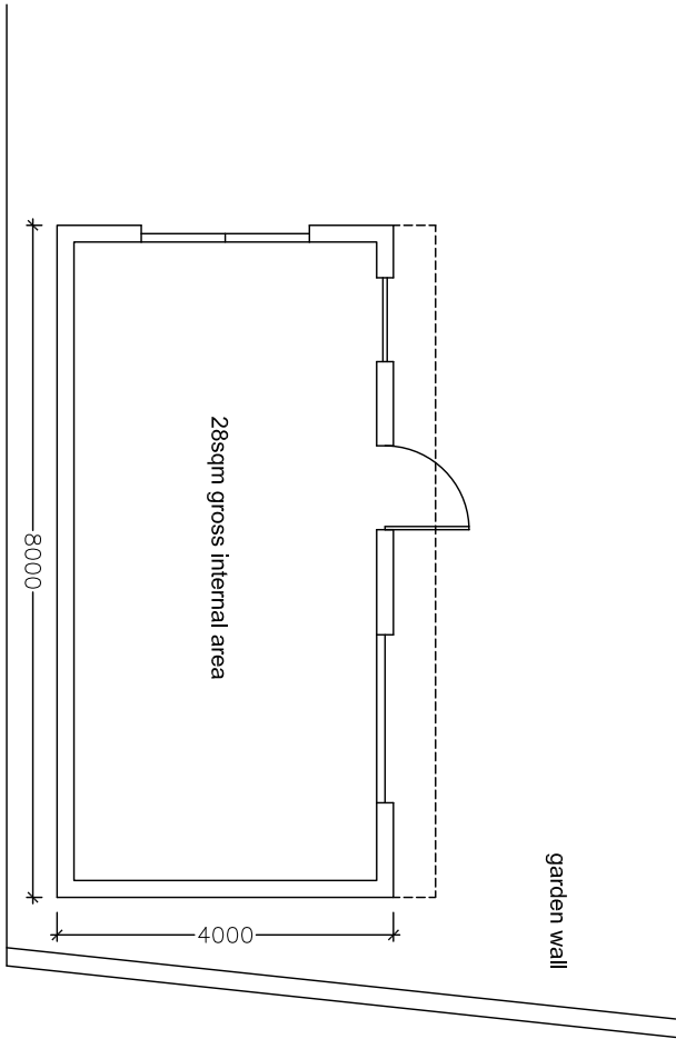
proposed plan 1:100
