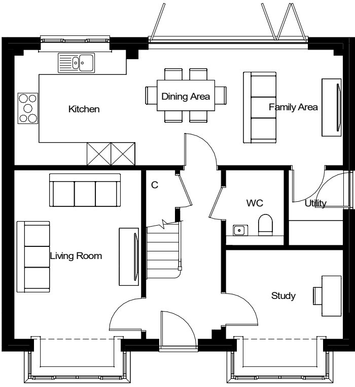
Ground Floor P006 - 4H4b
