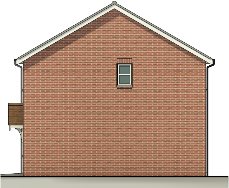
Right Elevation P009
