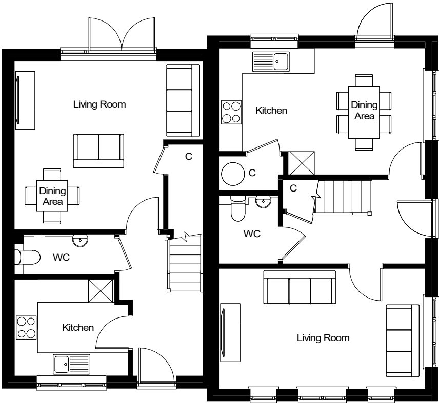
Ground Floor P018 - S2H1
