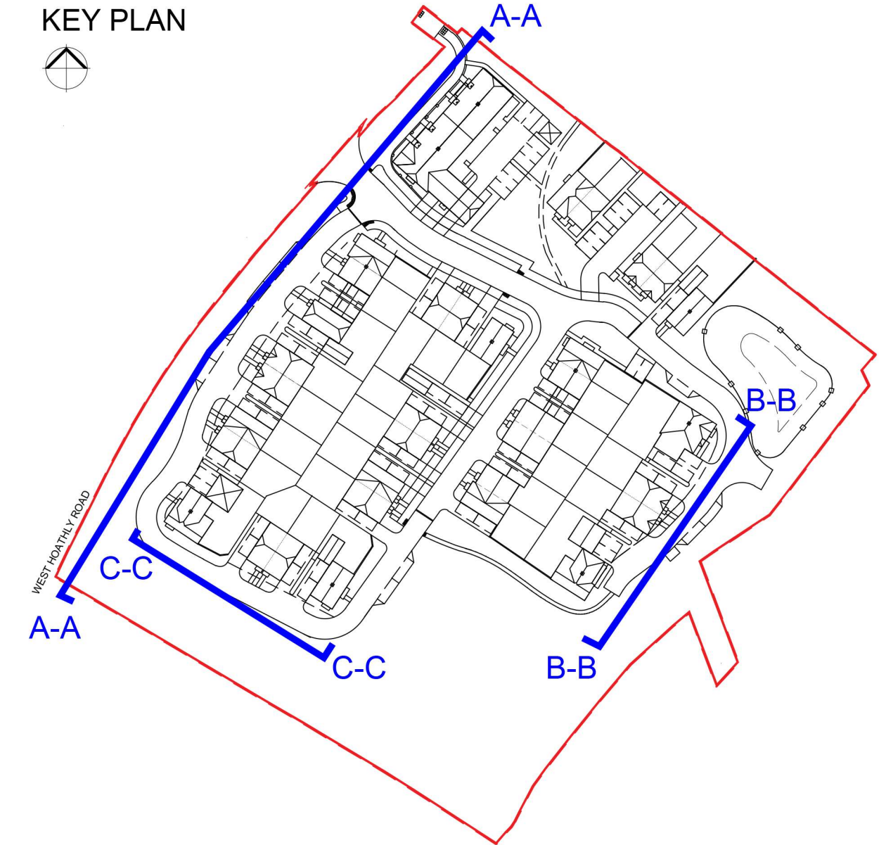
KEY PLAN
