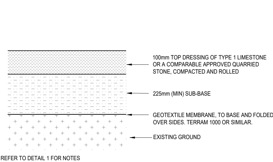
BRIDLEWAY SURFACE 'STANDARD TYPE' CONSTRUCTION DETAIL 4C FULL DEPTH
