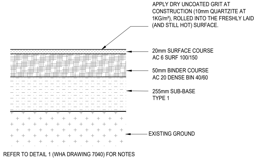
BRIDLEWAY SURFACE 'SPRAY AND CHIP TYPE' CONSTRUCTION DETAIL 4D FULL DEPTH
