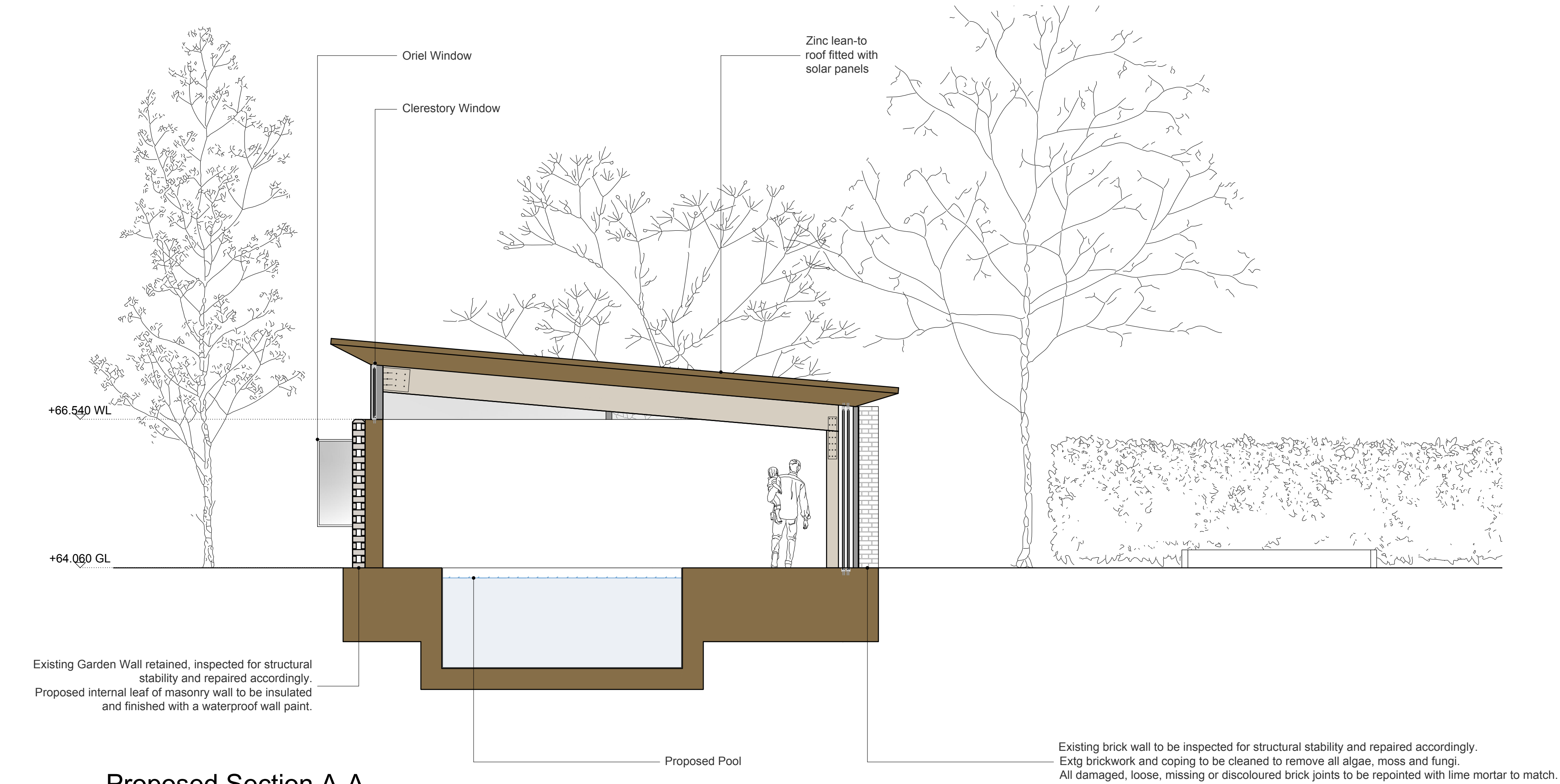
01 Proposed Section A-A 1:50 @ A1 ; 1:100 @ A3
