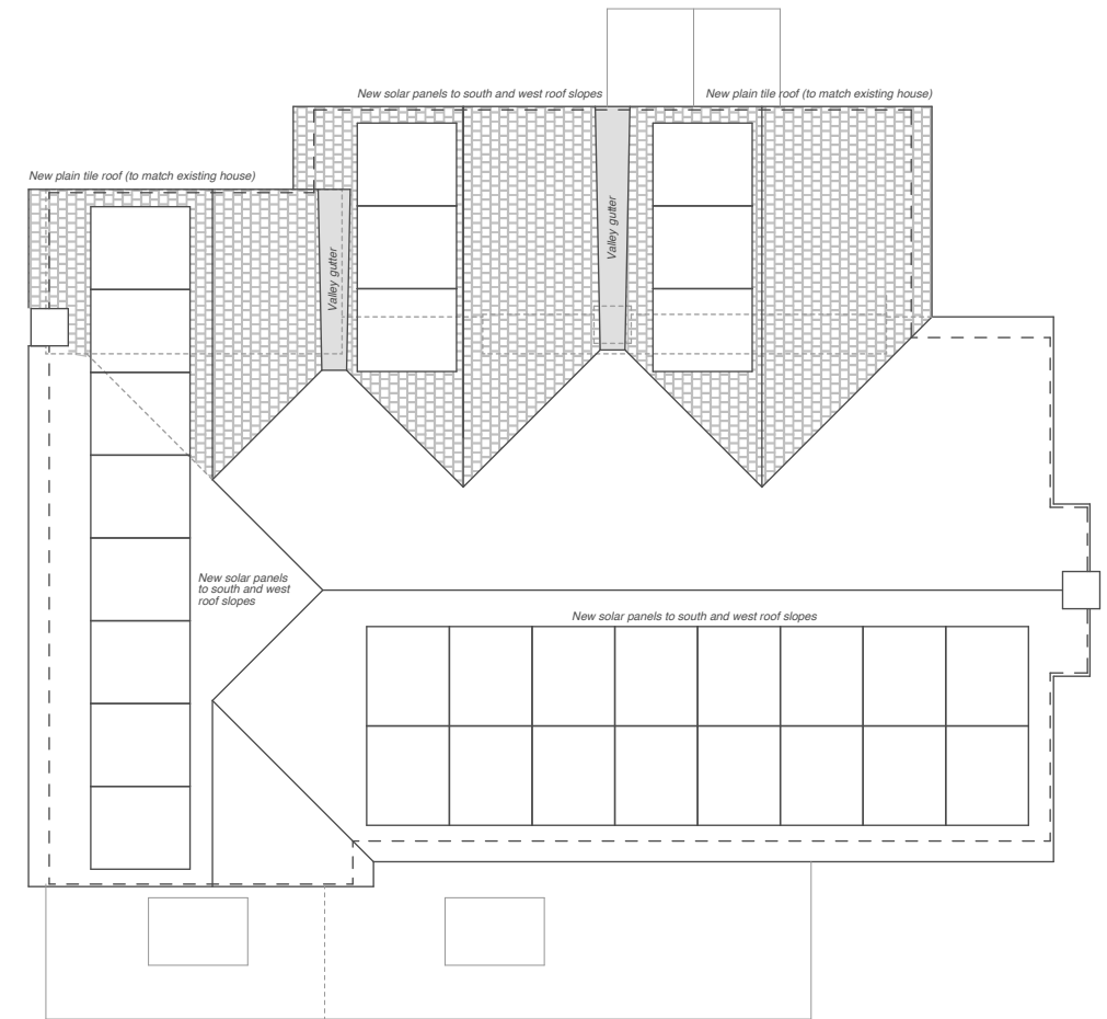
ROOF PLAN 1:100
