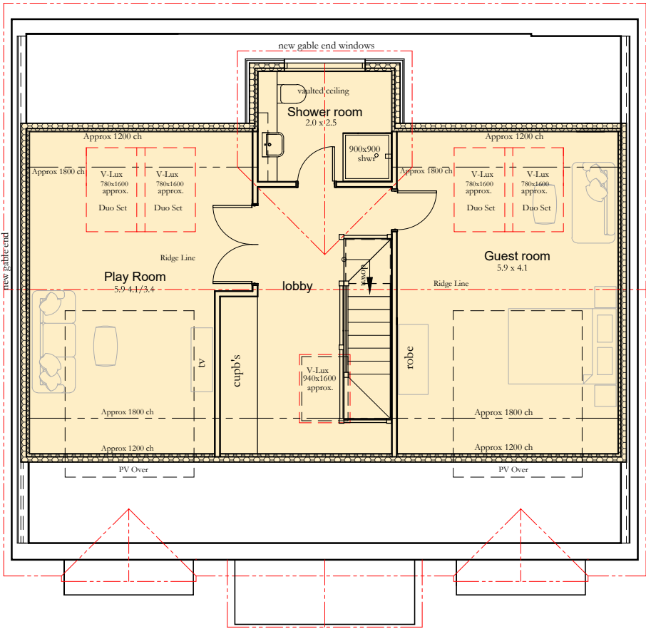
PROPOSED PLAN- LOFT FLOOR SCALE 1 : 100 @ A3
