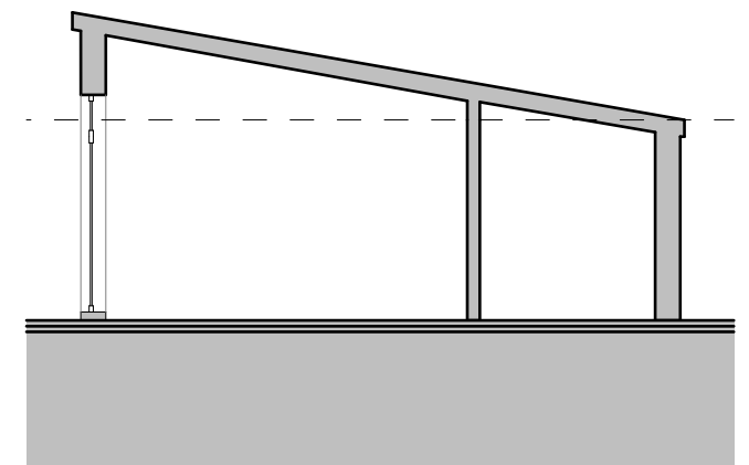
PROPOSED SECTION 1:100
