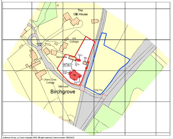
SITE LOCATION PLAN - AS PROPOSED SCALE @ 1:1250 ON AN A1 SHEET
