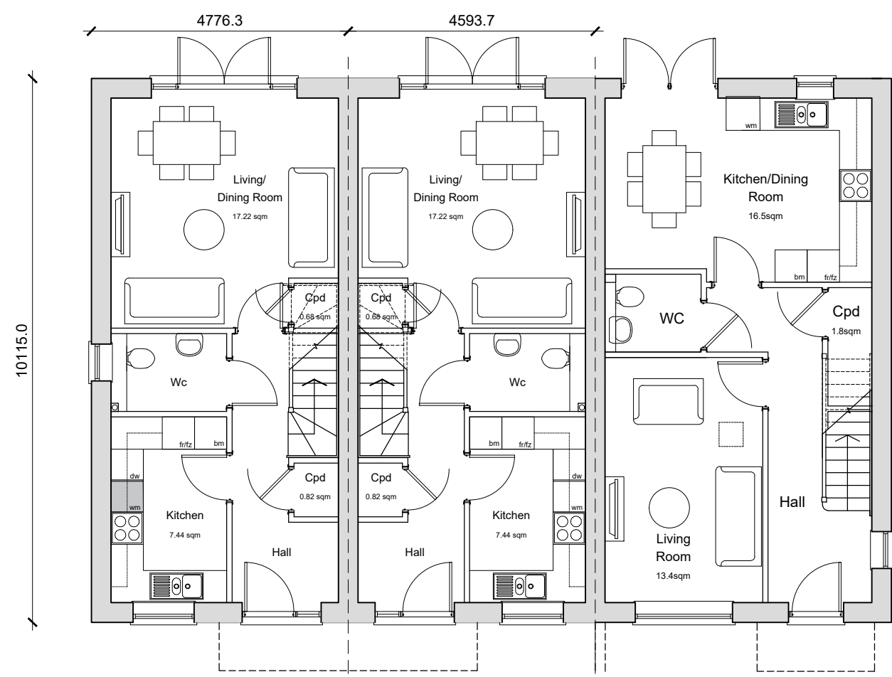
Ground Floor Plan HT21-HT21 2-Bedroom 4-Person House 79.36sqm / 854sqft GFA (to finished) A minimum of 2 days storage provided in accordance with NDIS requirements. Plots 18-19-20
