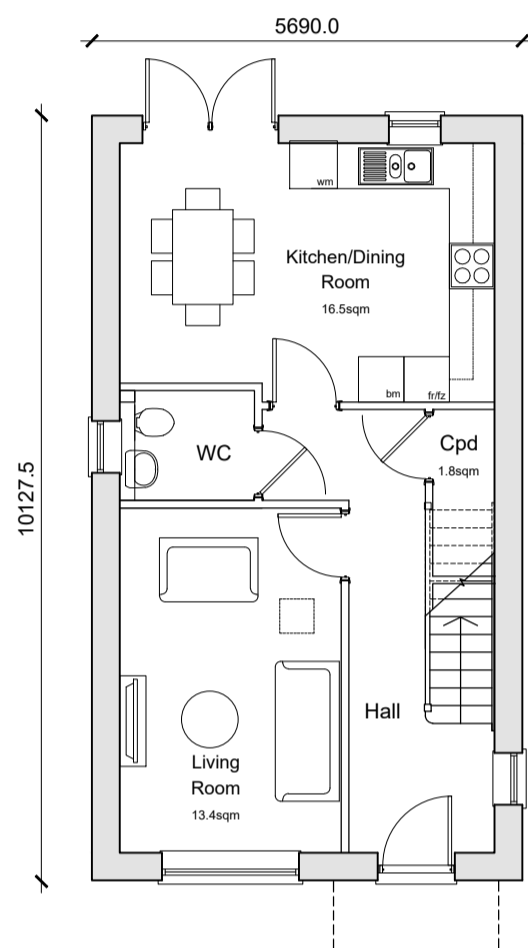
Ground Floor Plan HT31 3-Bedroom 5-Person House 55.0sqm (1180sqft) GFA, (to include) A minimum of 2.5 sqm storage provided in accordance with NDIS requirements.
