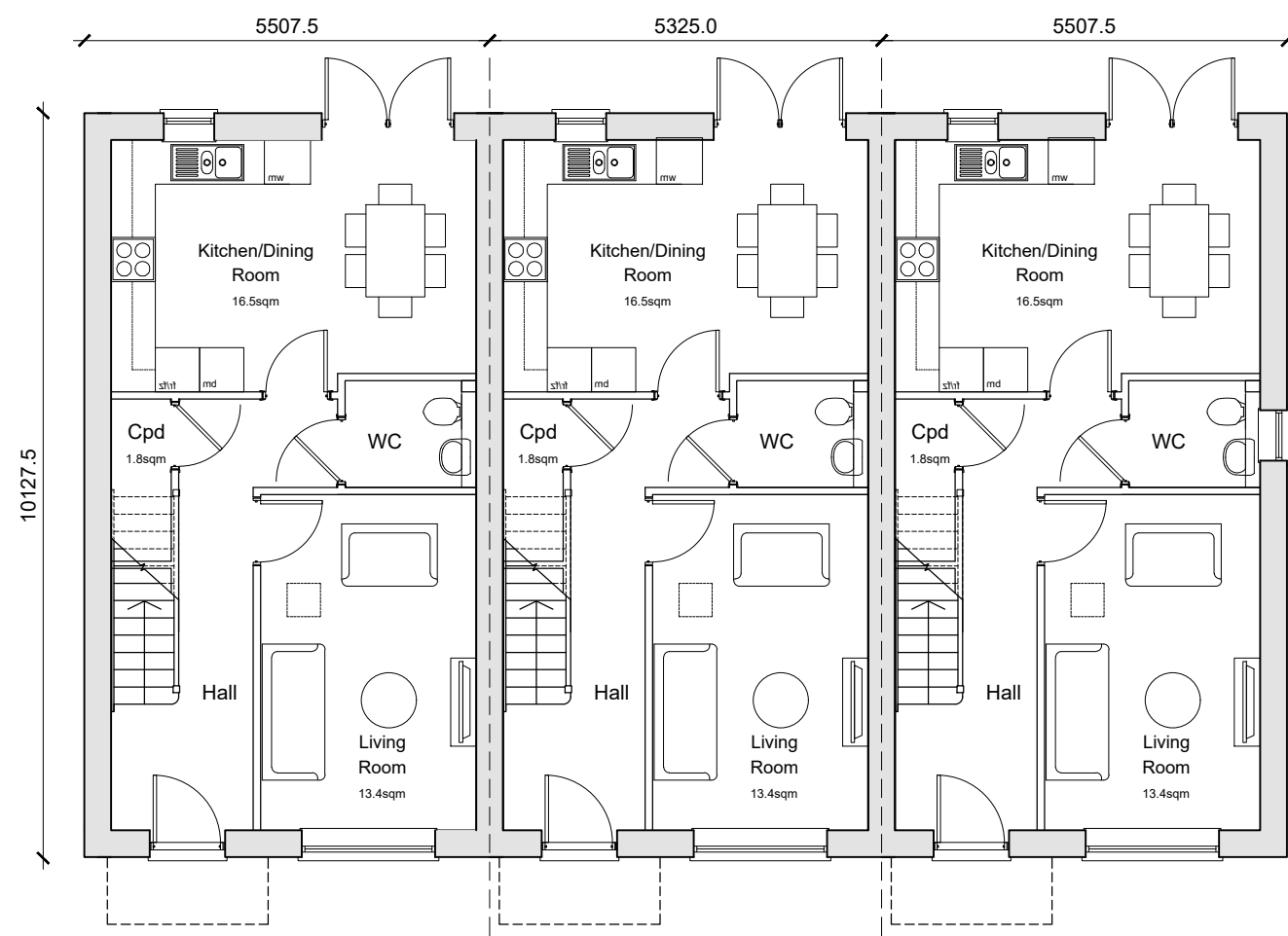
Ground Floor Plan HT31 3-Bedroom 5-Person House 83.58sqm / 1002sqft GFA (in-house) A minimum of 2.5 ton storage provided in accordance with NDIS requirements.
