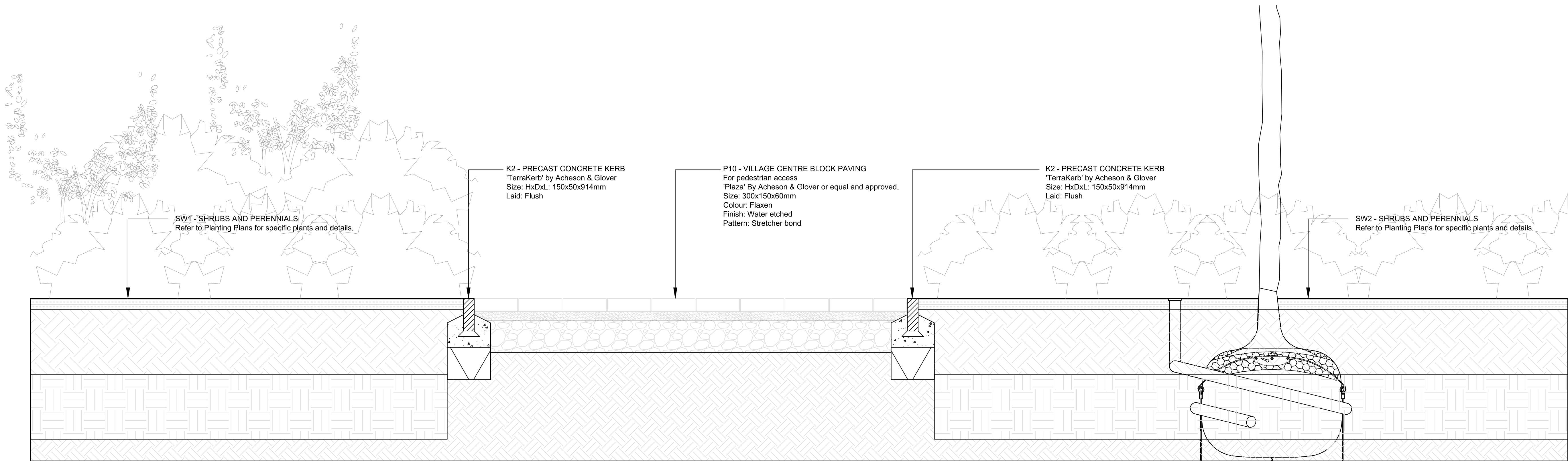
02 | PAVING AND KERB INTERFACE SECTION 1:10
