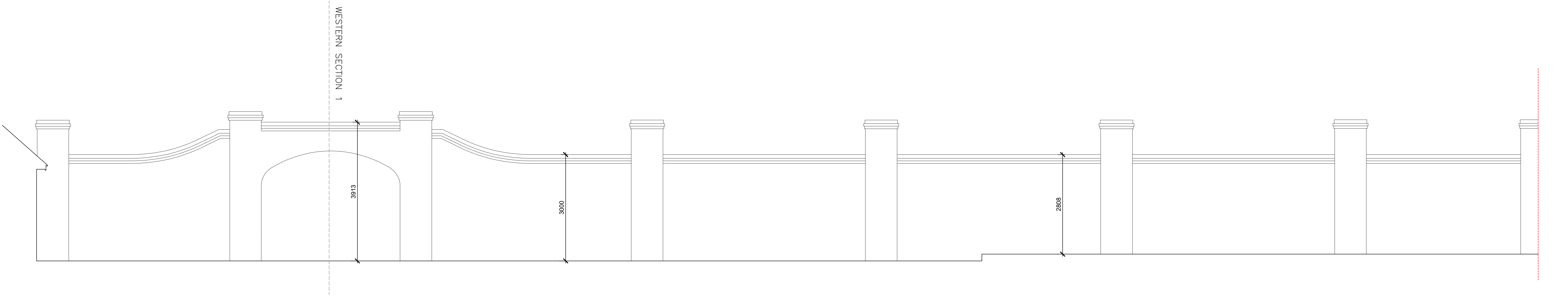
South West Wall Part 1 - Existing - 1:50@A0
