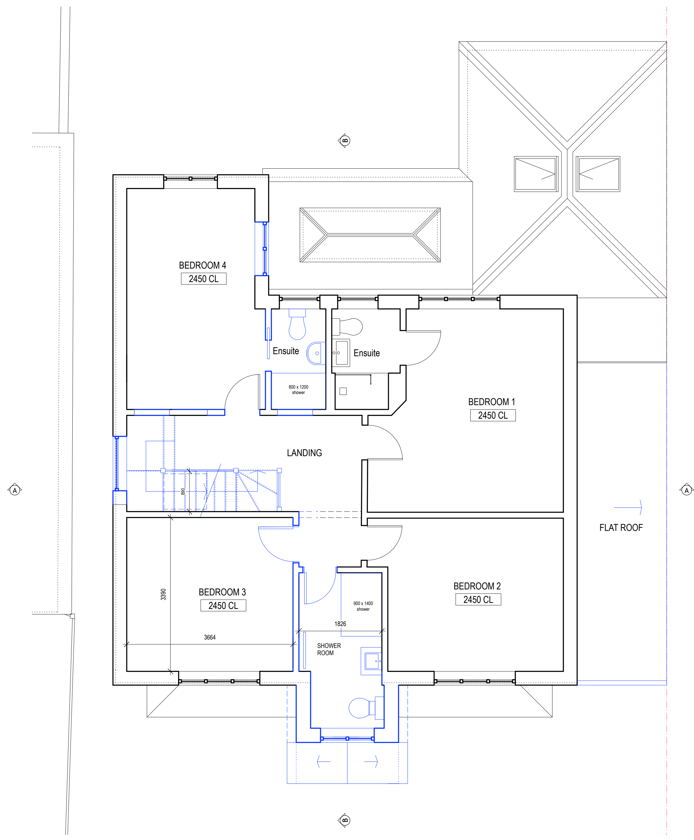
1F PLAN
