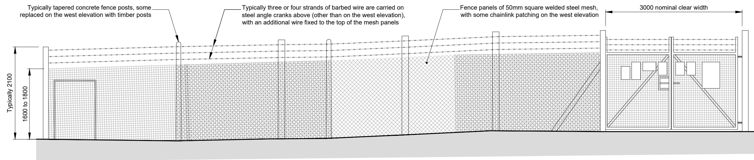
Existing Elevation
