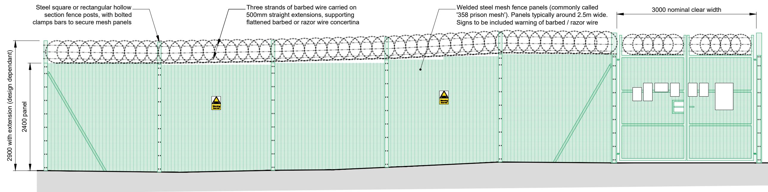
Illustrative Upgraded Elevation
