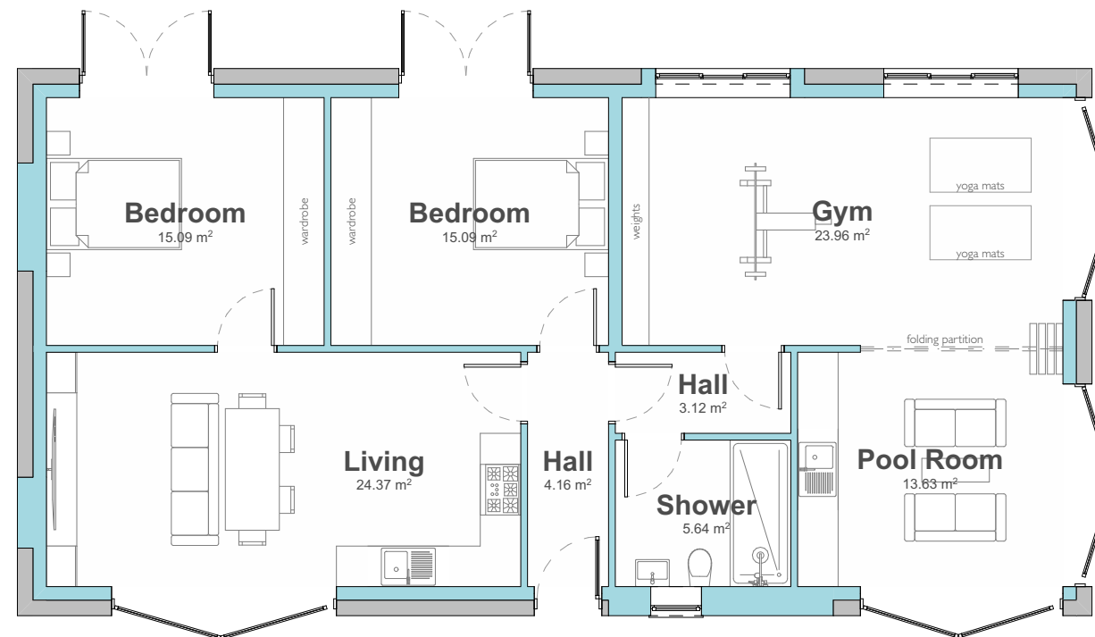
Proposed Annex Ground Floor Plan
