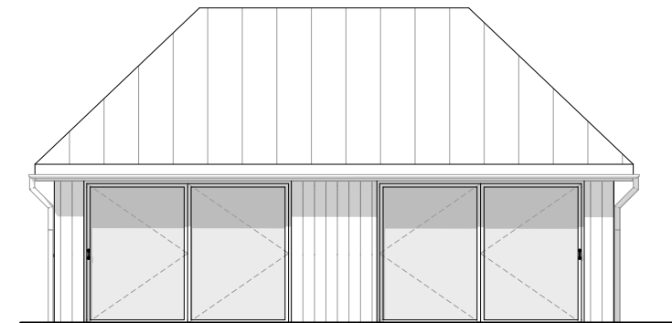
Proposed Side (East) Elevation
