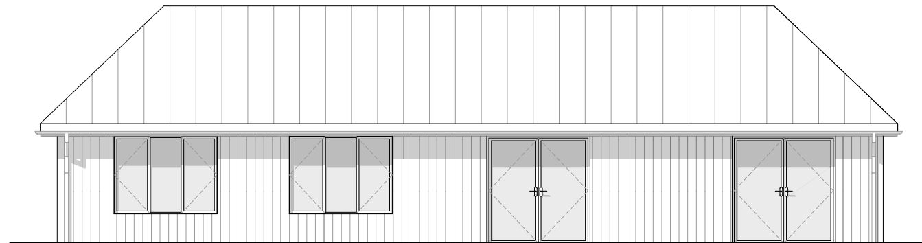
Proposed Rear (North) Elevation
