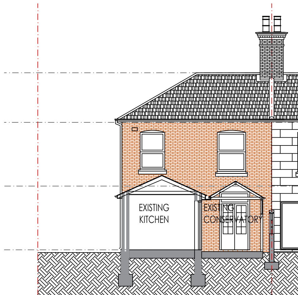
EXISTING SECTION A-A
