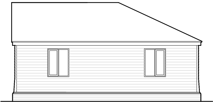
PROPOSED SIDE ELEVATION South facing
