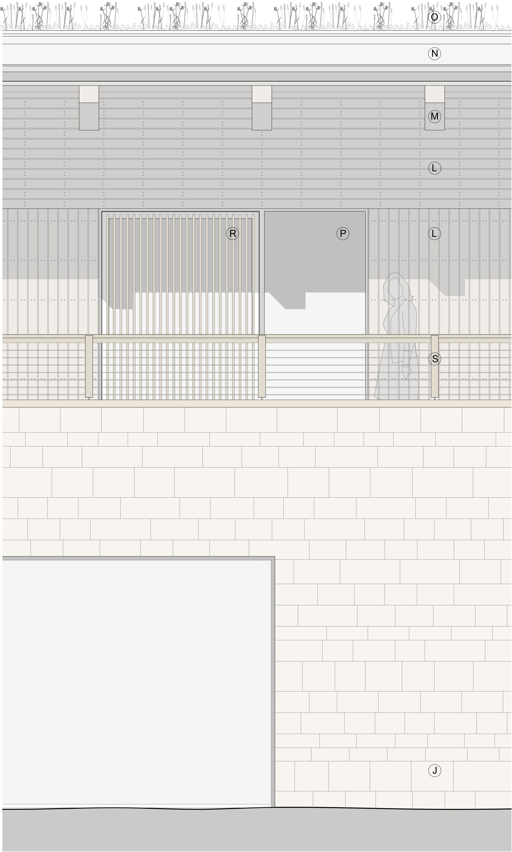
Proposed Detail Elevation 1:20
