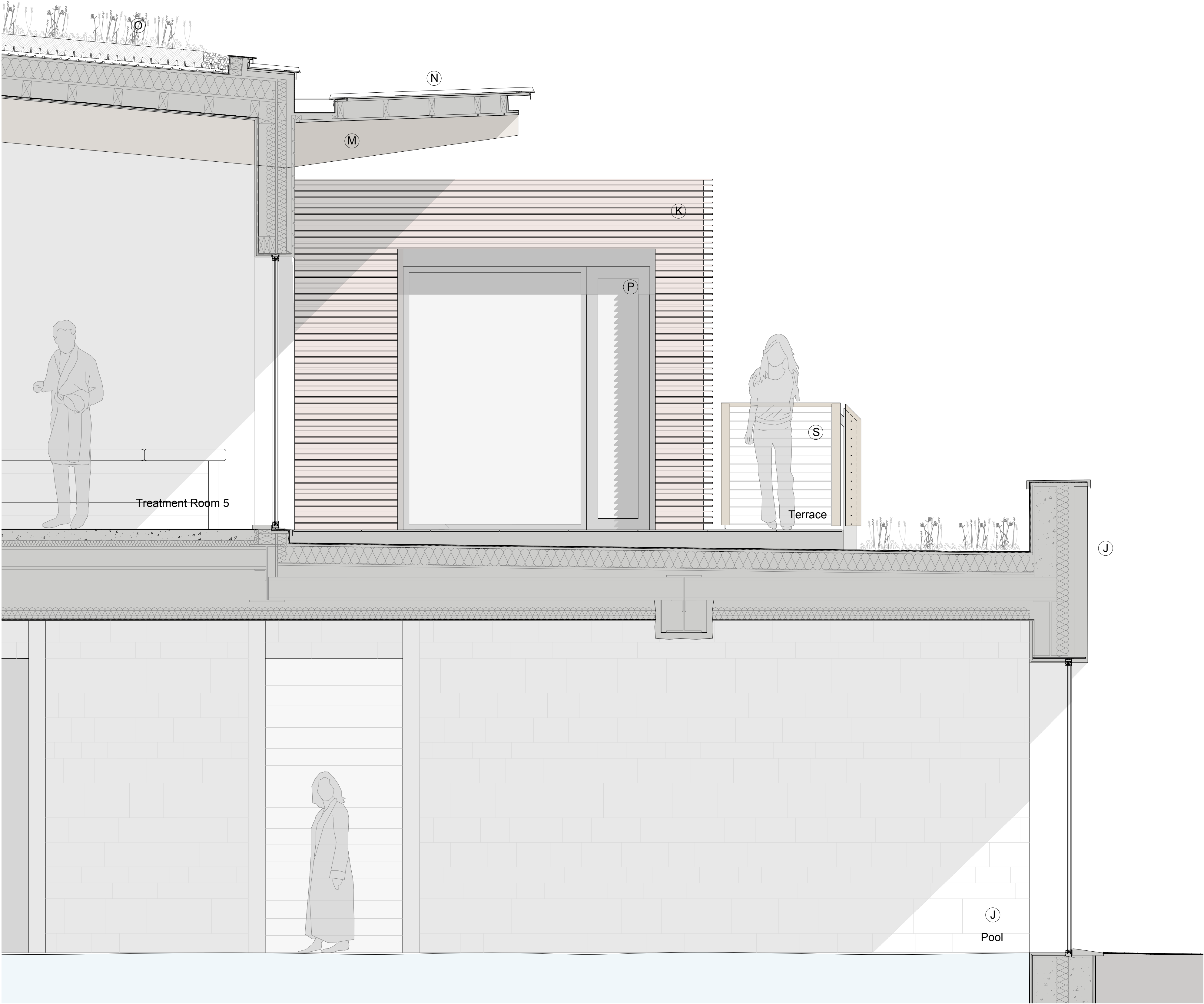
Proposed Detail Section 1:20
