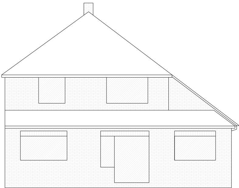
South Elevation
