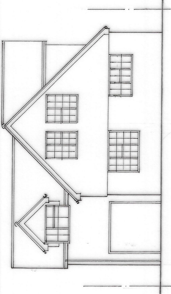
FRONT ELEVATION 1.100
