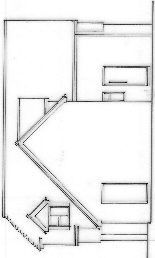
LEFT SIDE ELEVATION 1.100 (EXISTING AND PROPOSED)
