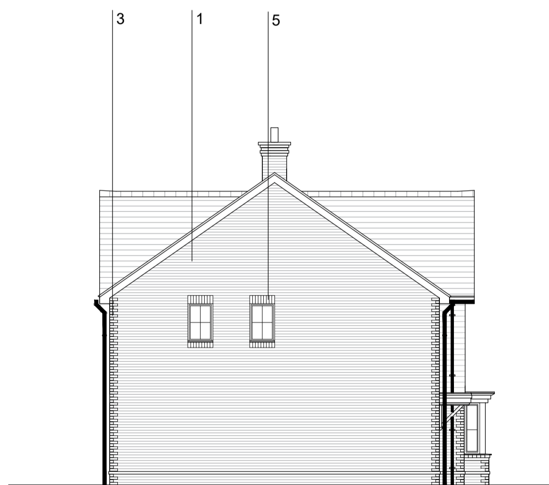
SIDE ELEVATION
