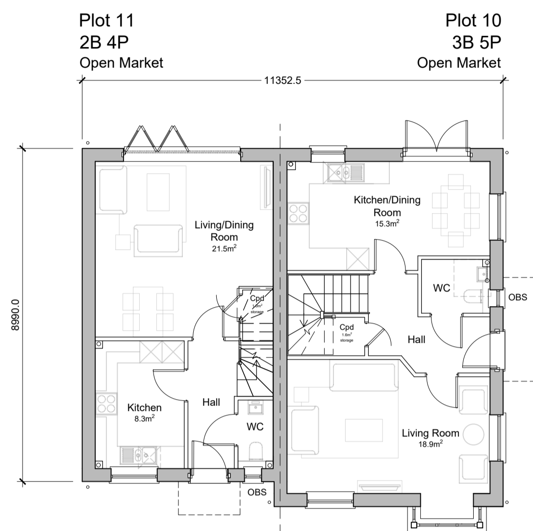
GROUND FLOOR
