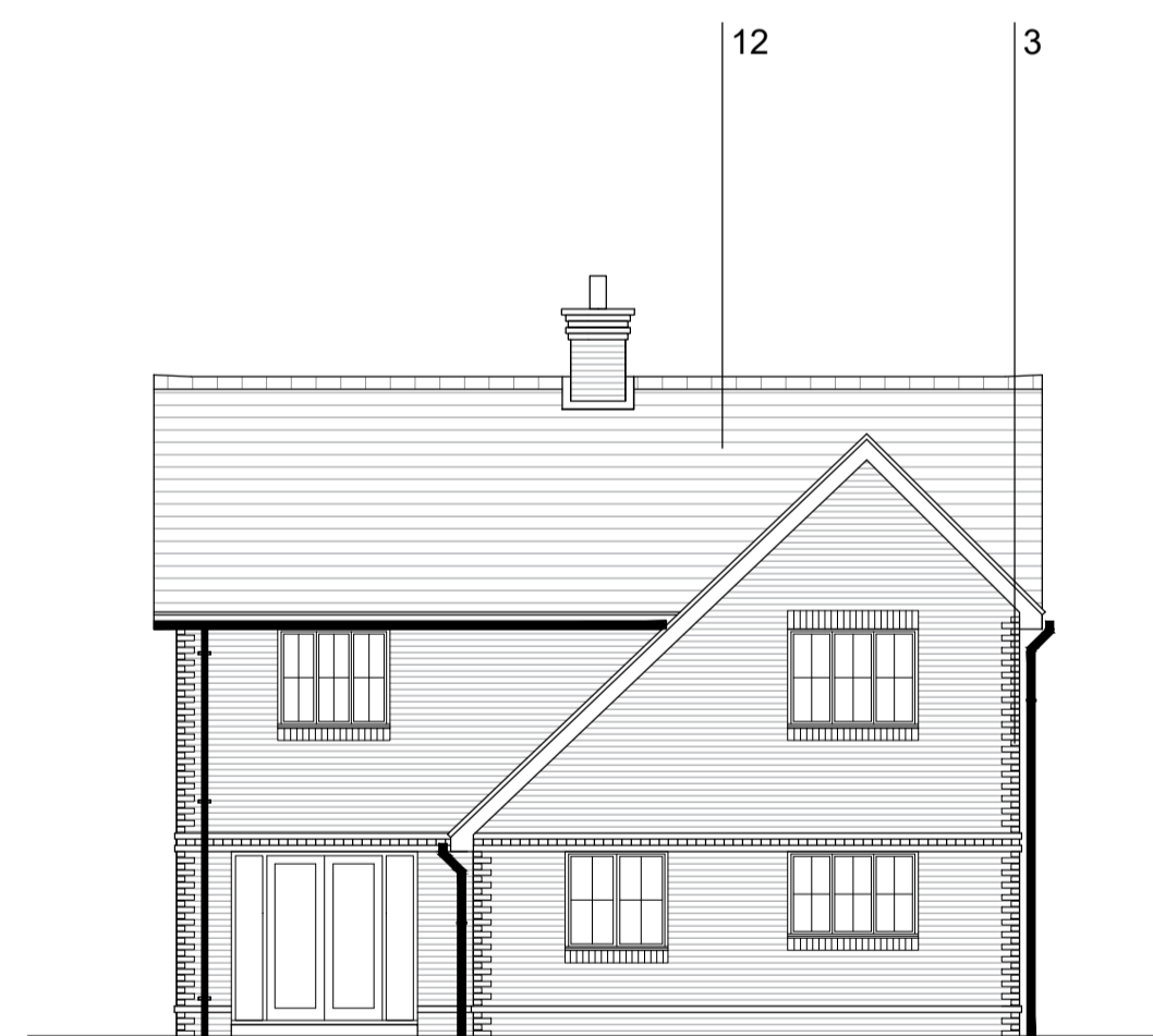
REAR ELEVATION
