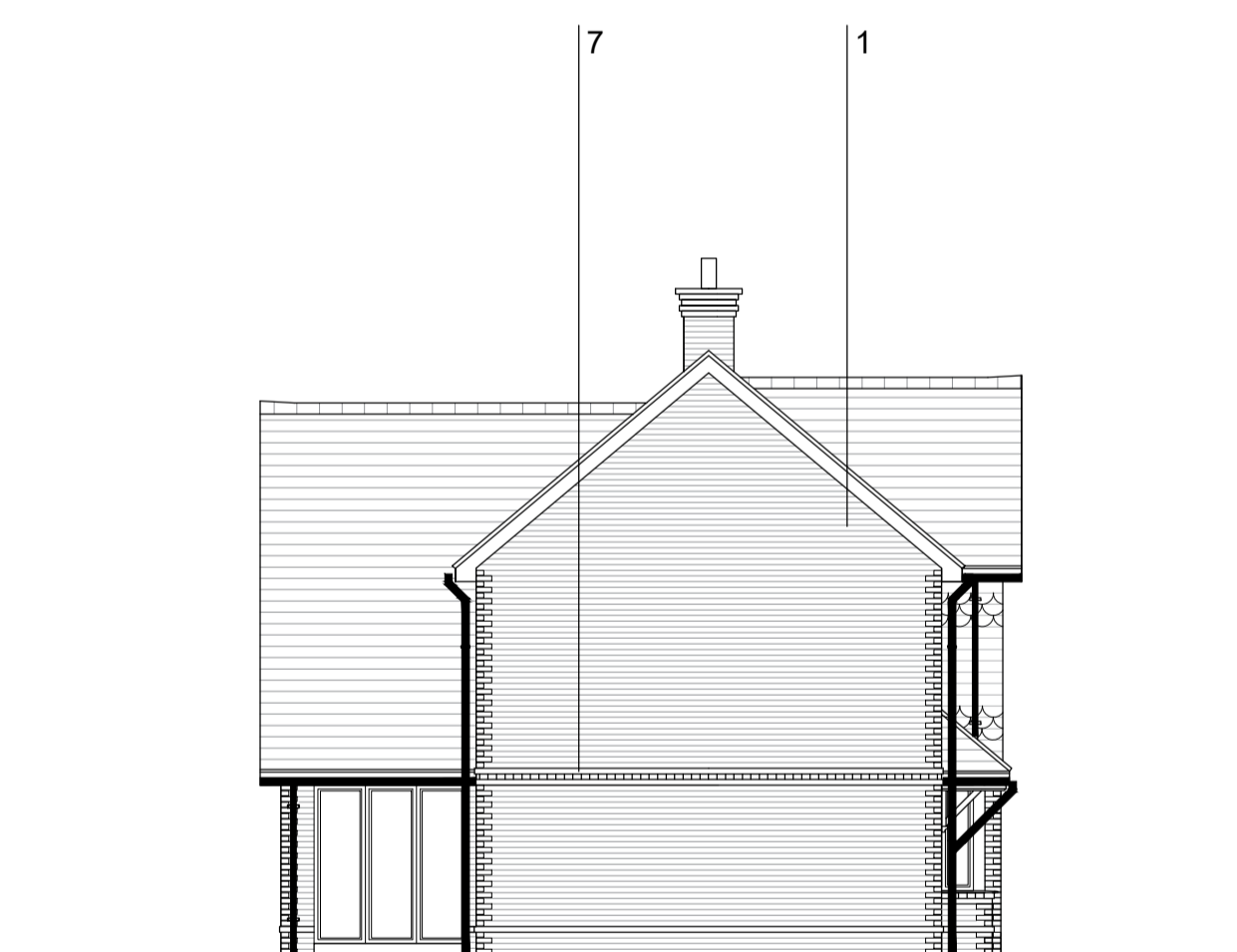
SIDE ELEVATION
