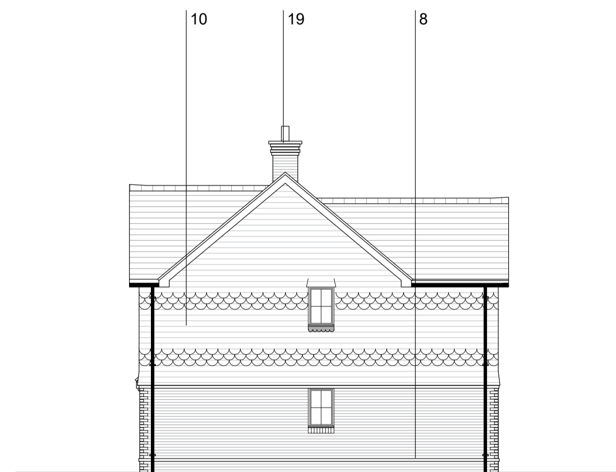
SIDE ELEVATION
