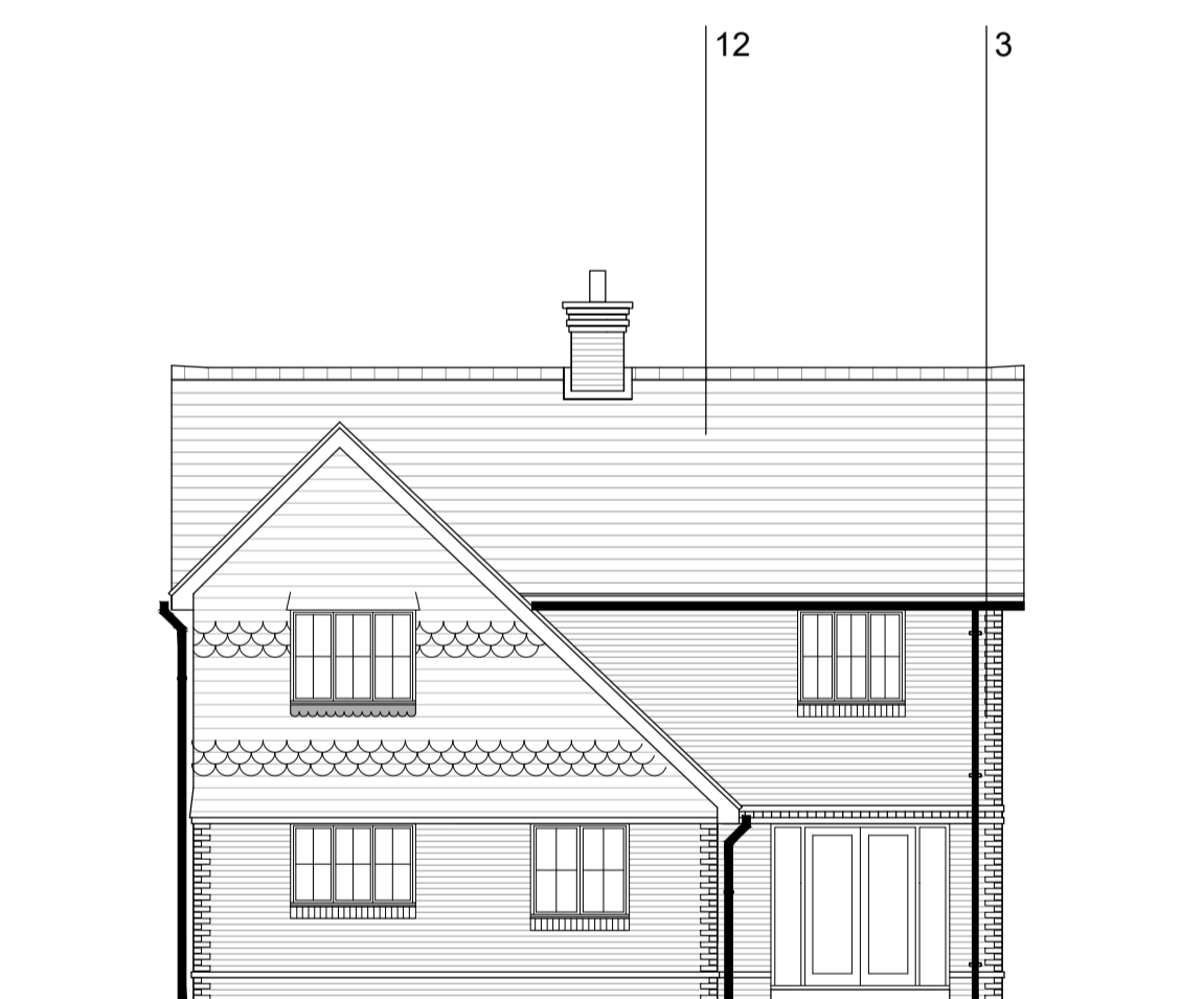
REAR ELEVATION
